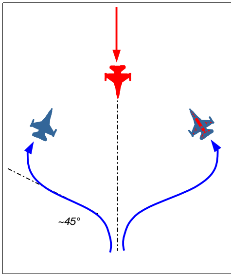
WIDE AZIMUTH BRACKET
